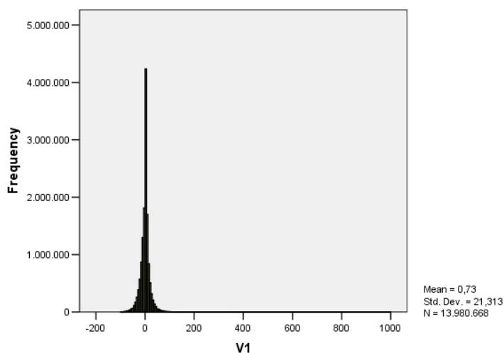
Slika 8. Histogram razlika DMR4x5–SRTM3x3
