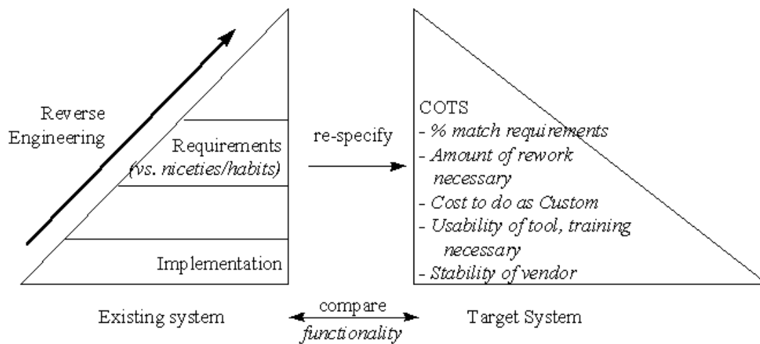
Fig. 3: COTS Track Hybrid Re-engineering
