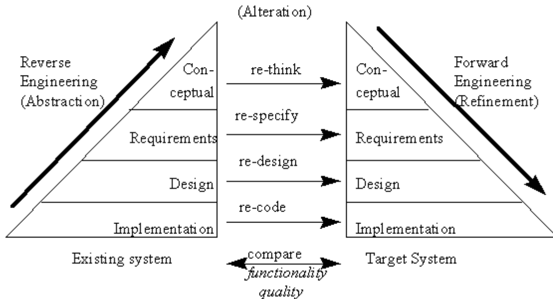
Fig. 1: General Model for Software Re-engineering
