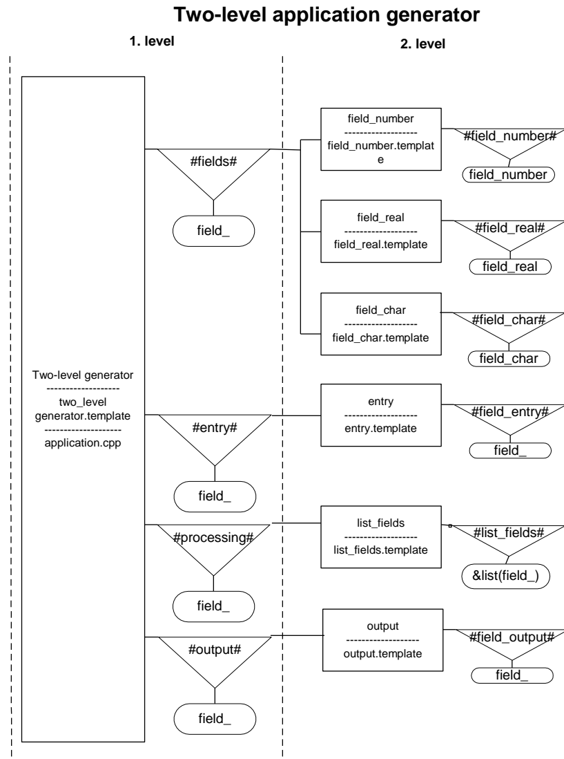
Fig. 8: The metascripts diagram of two-level application generator from the example
