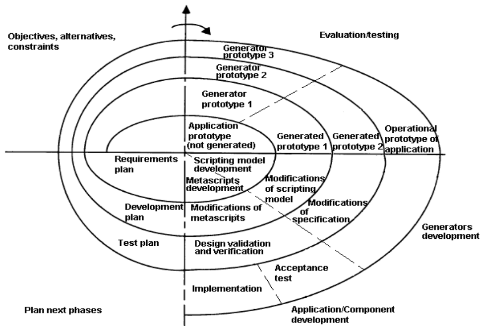
Fig. 12: Generative application development as spiral development using the Boehm (Boehm, 1988) model
