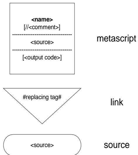
Fig. 6: Elements of the metascripts diagram
