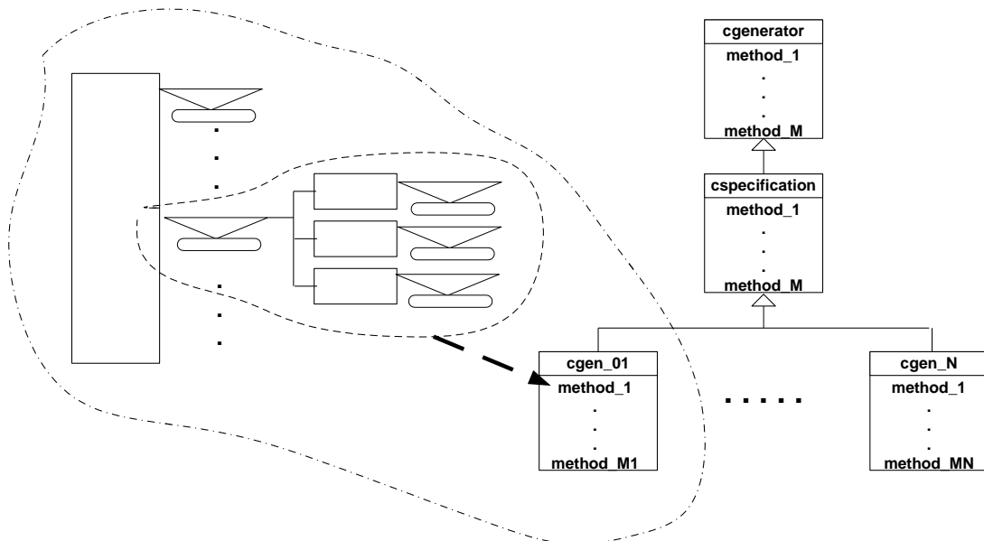
Fig. 11: General structure of generator based on C++ generative objects
