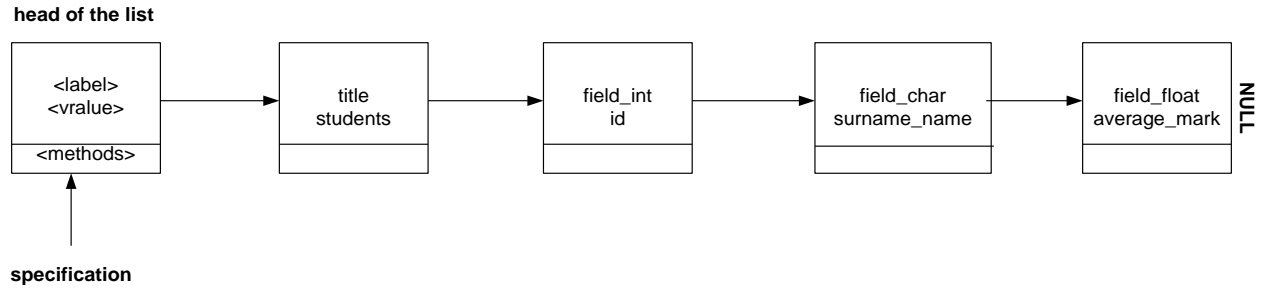
Fig. 10: Linked list of specification
