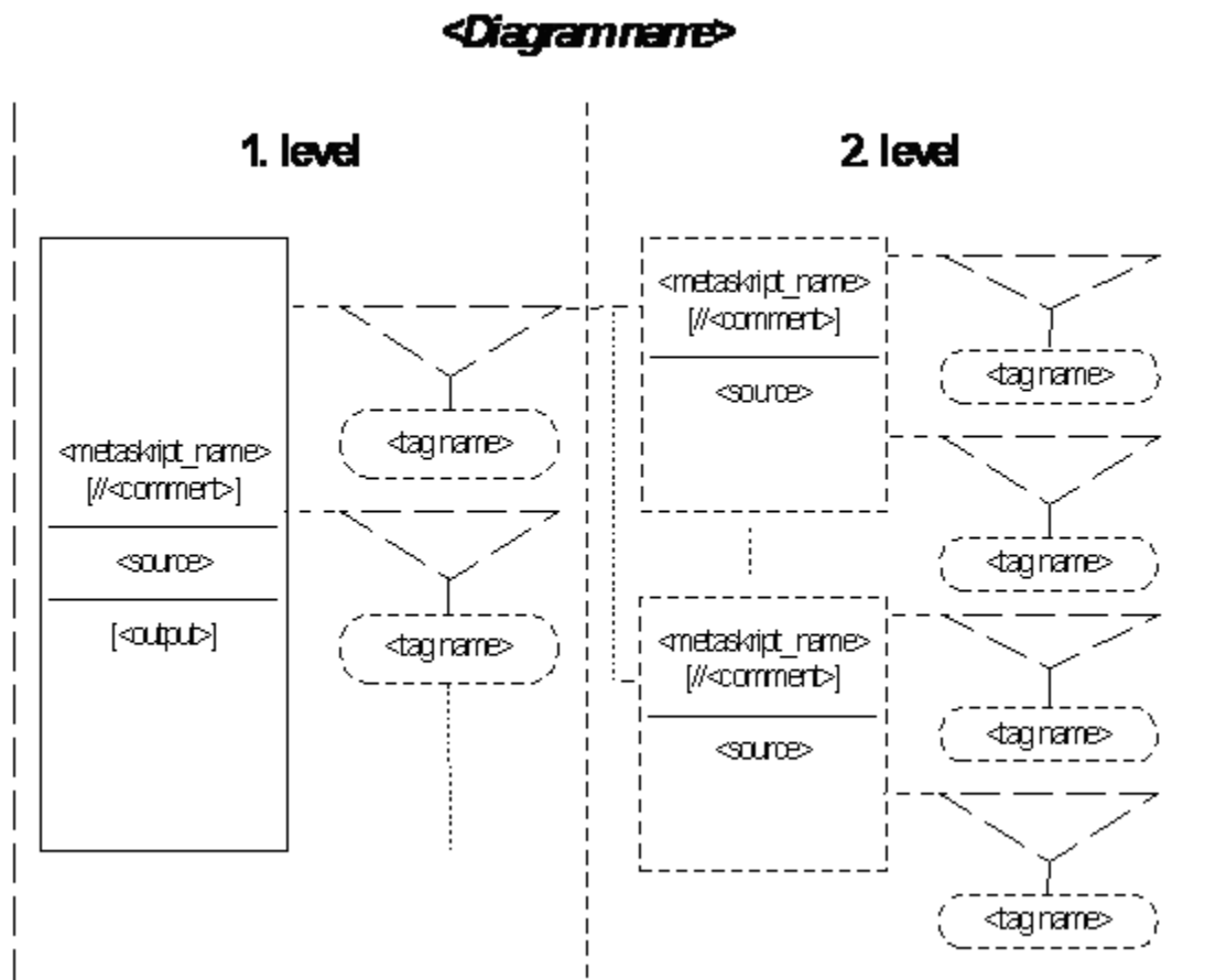
Fig. 7: Structure of metascripts diagram
