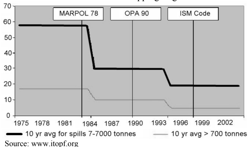
Figure 6. Ten-year Averages for the Number of Tanker Spills in Relation to the Introduction of Shipping Regulations
