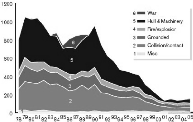
Figure 8. Tanker incidents by cause 1978-2005
