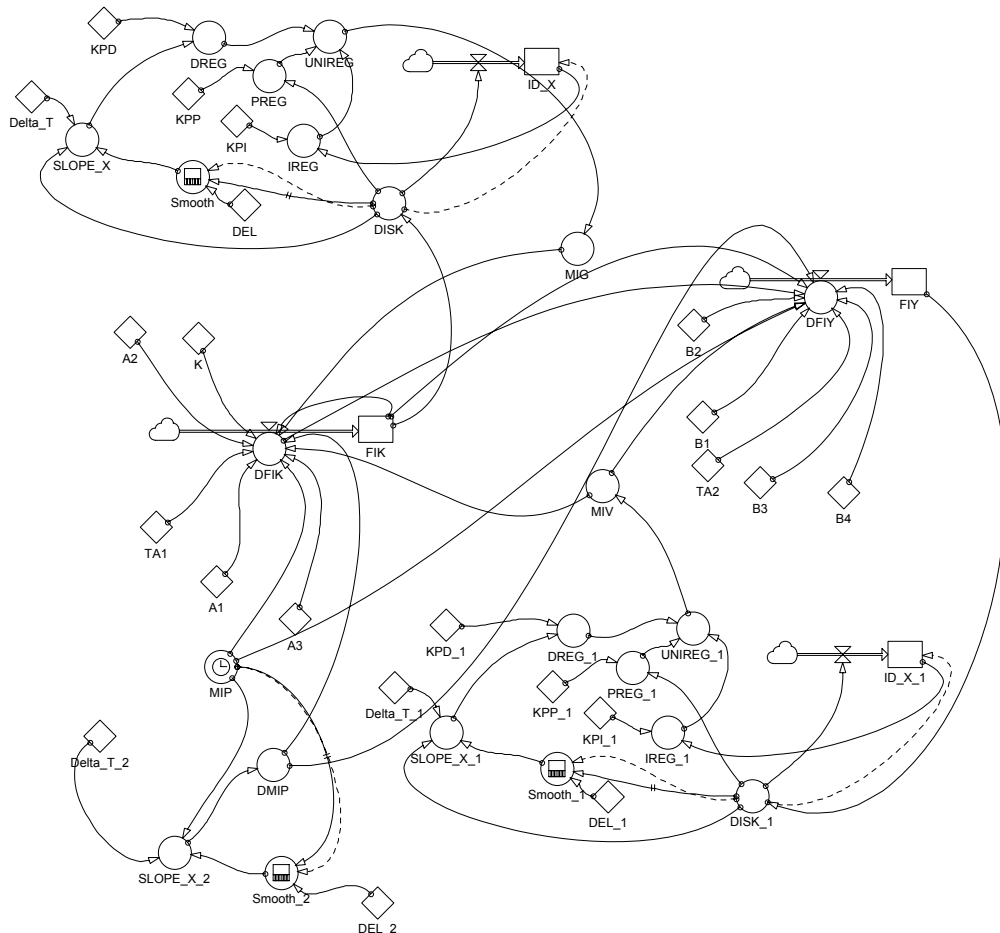
Sl. 5. Globalni dijagram toka brodskoga parnog kotla s ugrađenim PID-regulatorima Fig. 5. Global diagram of the flow of vessel's steam boiler with PID regulators installed
