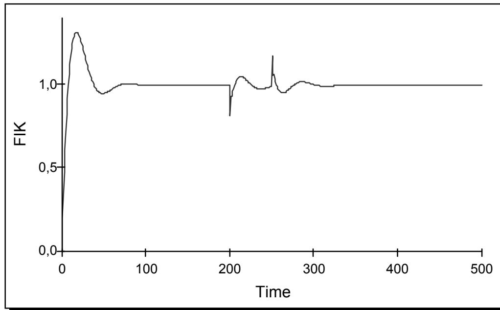
SI. 6. Relativno stanje tlaka pare u parnom kotlu Figure 6. Relative condition of the pressure of the steam in the steam boiler
