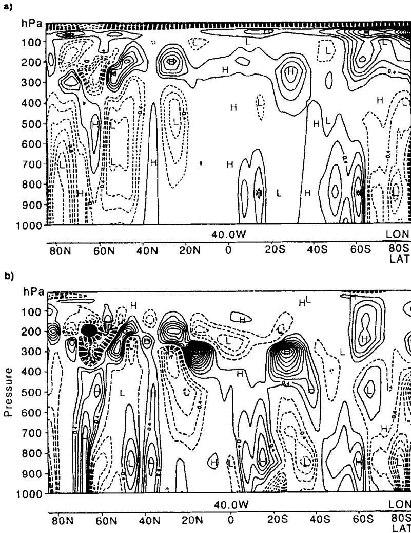
Figure 8. North-south cross-section along 40^{\circ}\text{W} of analysis increments of temperature (K) at 00 UTC 16 August 1993 for analyses without TOVS or SATEM data: (a) 3D-Var; (b) OI. Contour interval 0.2 K.
