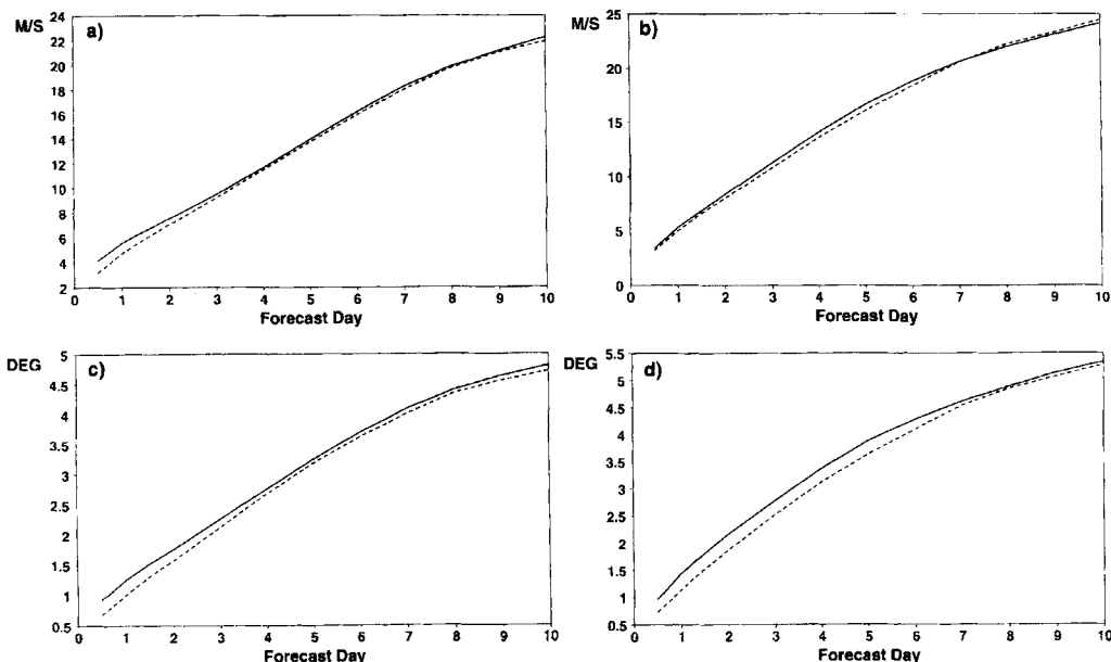
Figure 2. Average r.m.s. errors of forecasts of wind ( m s^{-1} ) and temperature (K) at 200 hPa, averaged over 120 days at 12 UTC in three separate periods (5 April 1995–14 May 1995; 24 August 1995–28 October 1995; 16 January 1996–29 January 1996), verified against their own analyses: (a) northern hemisphere wind; (b) southern hemisphere wind; (c) northern hemisphere temperature; (d) southern hemisphere temperature. The full line denotes OI and the dashed line 3D-Var.
