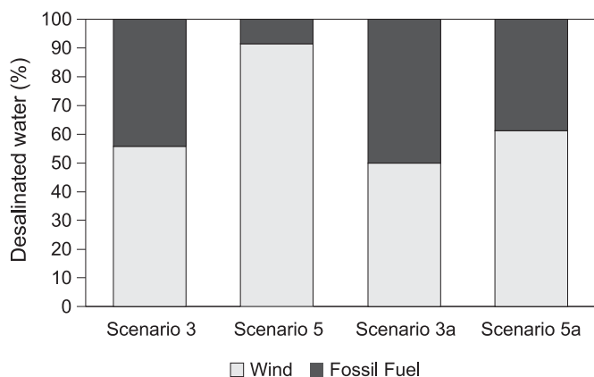
Fig. 9. Production of desalinated water in S. Vicente in 2020 for different scenarios.
