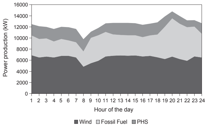
Fig. 7. Production in 2020 for Scenario 4.
