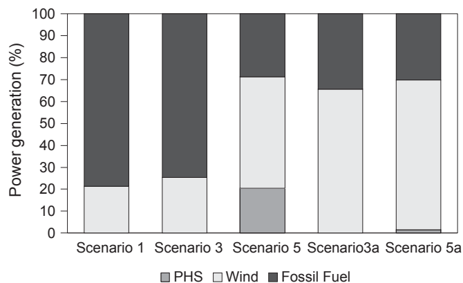
Fig. 8. Power production in S. Vicente in 2020 for different scenarios.
