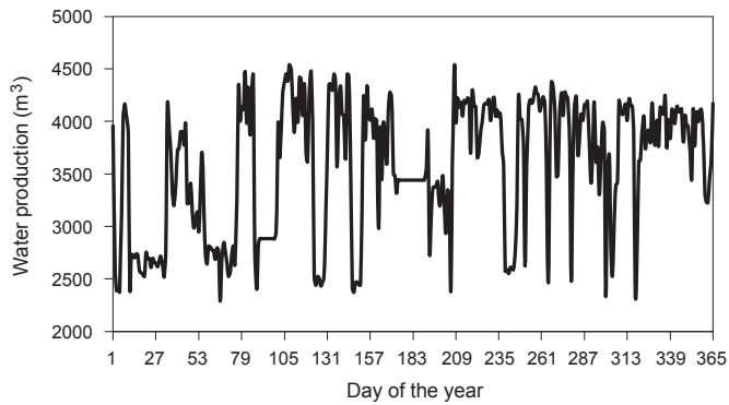
Fig. 4. Daily water production in S. Vicente in 2010.
