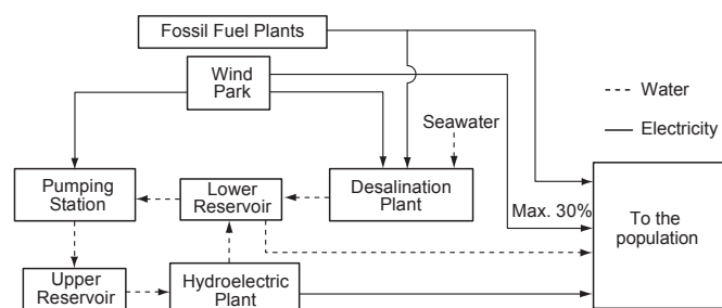
Fig. 5. Schematic diagram of Scenario 4.
