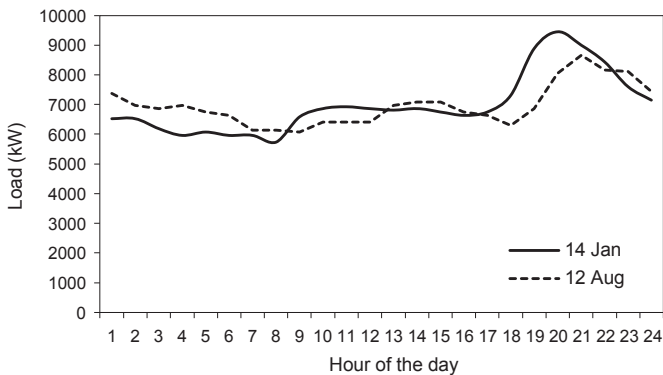
Fig. 3. Hourly electricity load of S. Vicente in a summer day and in a winter day in 2010.
