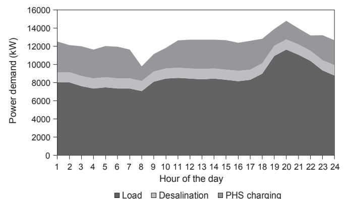
Fig. 6. Demand in 2020 for Scenario 4.
