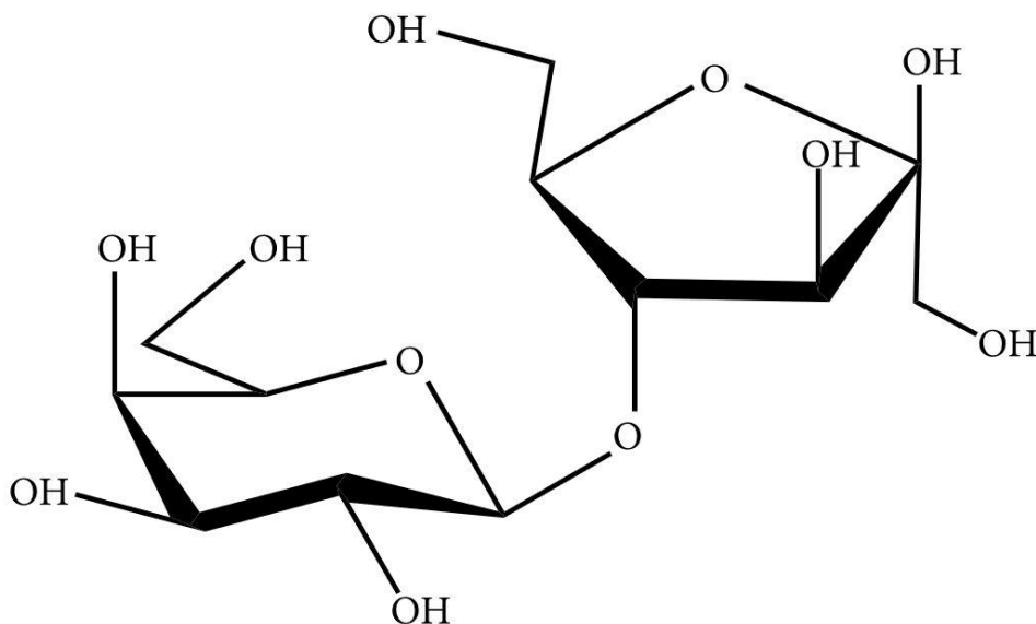
Figure 62 Lactulose structure (61)
